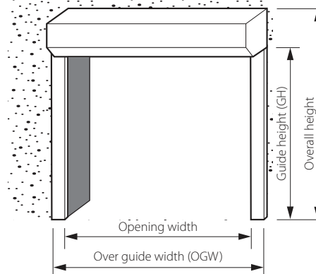
Width measurement guide
